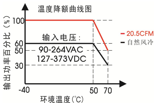
LOF350-20B12-C(满载 300W 带 20.5CFM 风扇)
