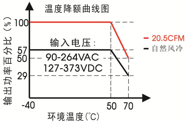
LOF350-20B24/27/48-C(满载 350W 带 20.5CFM 风扇)
