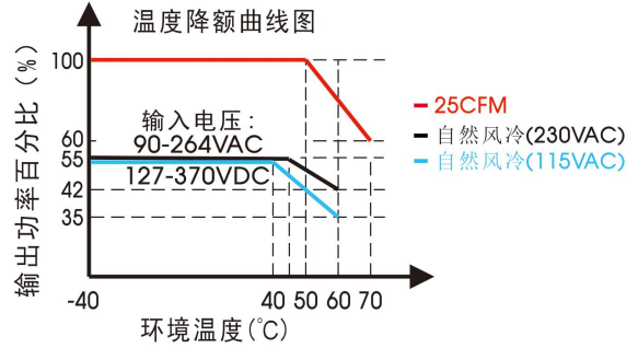
LOF450-20B24/27/36/48 (满载 450W 带 25CFM 风扇)
