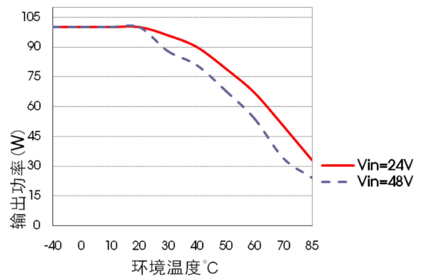
URF4812/15/24/48QB-100WFR3 温度降额曲线
