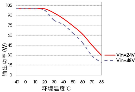
URF4812/15/24/48QB-100WR3 温度降额曲线
